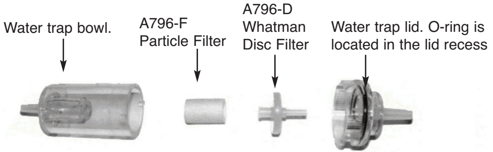
Exploded View of A796 Water Trap
